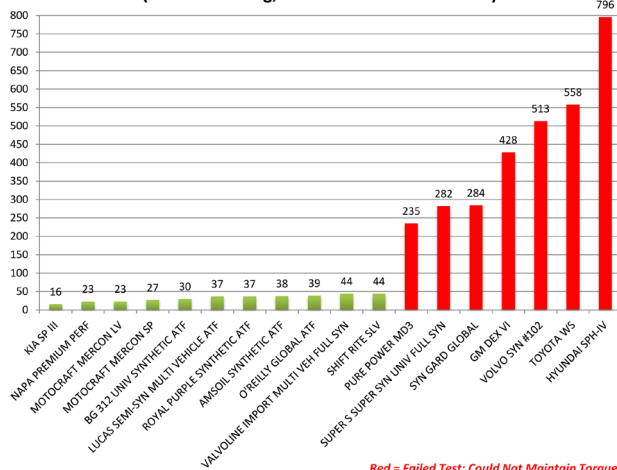
Automatic Transmission Fluid Wear Test Falex Wear Test ASTM D2670 (modified) (Mass loss in mg, after 3.5 hrs. at 500 ft. lbs.)
