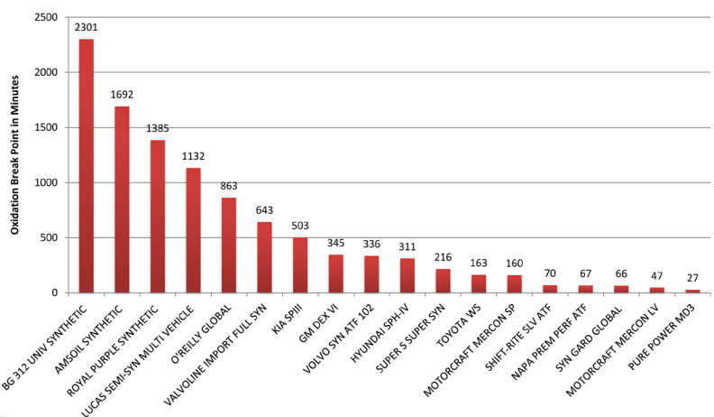
Automatic Transmission Fluid Oxidation Test (Thin Film Oxygen Uptake Test) TFOUT ASTM D4742
